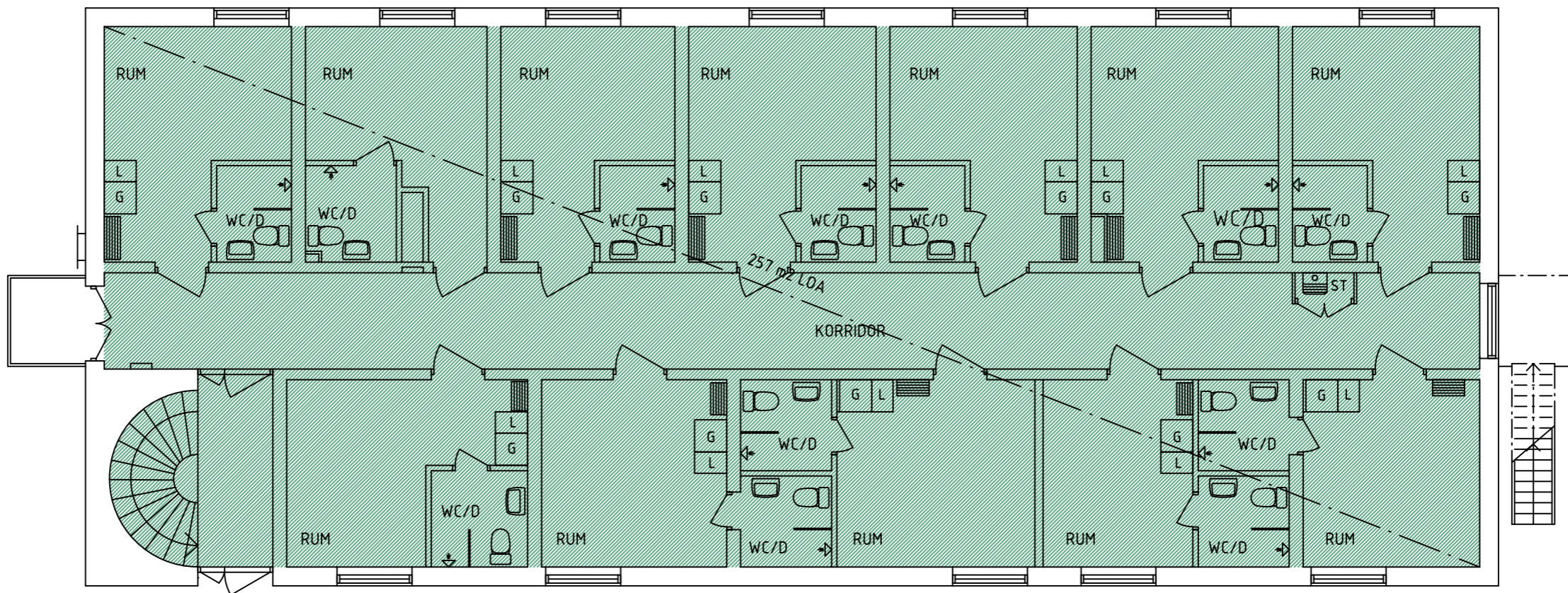
PLAN BV
